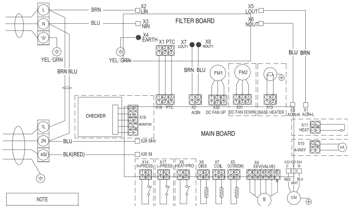
Electric Wiring Diagram 2219548.G
